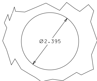
RECOMMENDED MOUNTING HOLE MAXIMUM PANEL THICKNESS: 0.68
